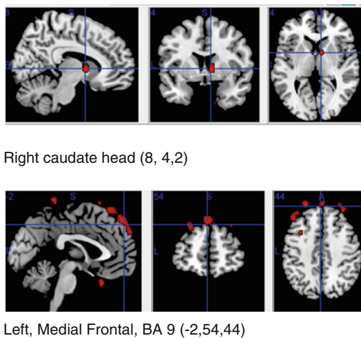
Fig. 3 Areas of GM decrease in BD patients in comparison with healthy controls (uncorrected P < 0.001 )
